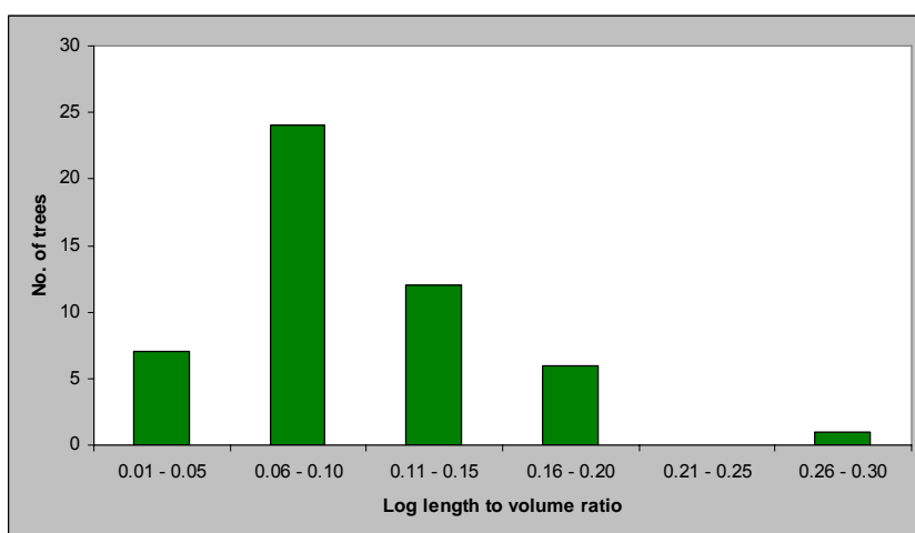
Figure 2: Distribution of trees in 'Log length to volume' ratios classes
