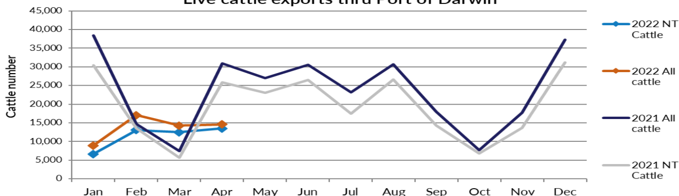
Live cattle exports thru Port of Darwin
